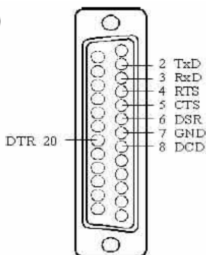
C104H/PCI DB25 Male (Opt4C)
